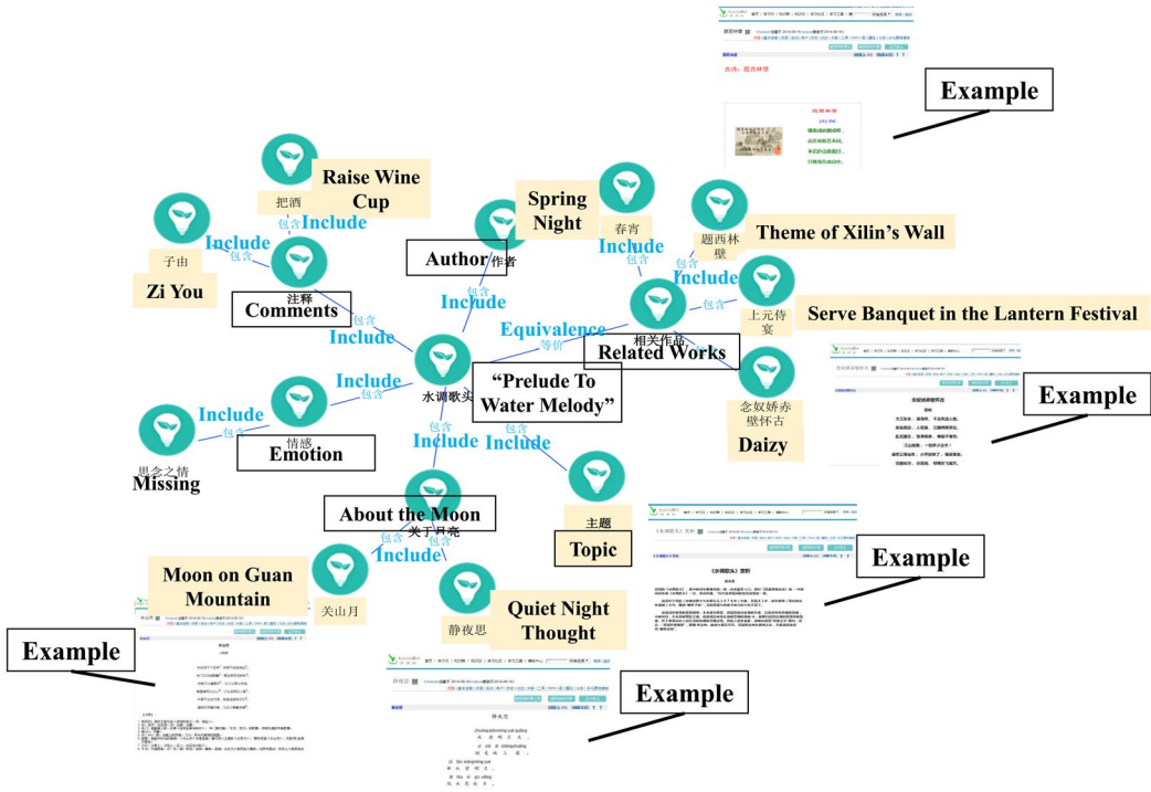
Figure 2: An individual knowledge graph based on the LCS
